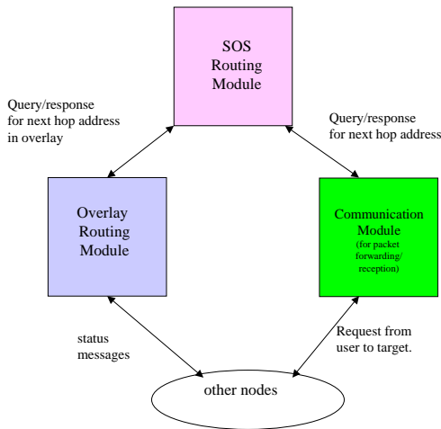
Figure 6: Software modules for the WebSOS implementation.
