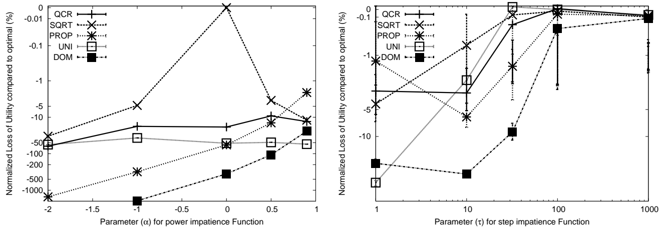
Figure 4: Comparison between QCR and several fixed allocations (homogeneous contacts): for power delay-utility function as a function of \alpha (left), for step delay-utility function as a function of \tau (right).
