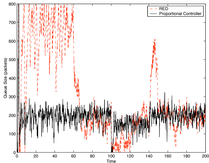
Fig. 6. Comparison of RED and the proportional Controller
