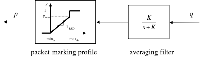
Fig. 3. RED as a cascade of low-pass filter and nonlinear gain element.
