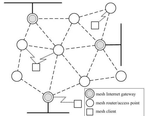
Fig. 1. Wireless mesh network architecture
