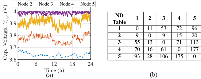
Fig. 8. Panda-D experimental evaluation for non-homogeneous power harvesting with N = 5 over 24 hours: (a) Capacitor voltage, V_{cap} , and (b) resulting neighbor table.
