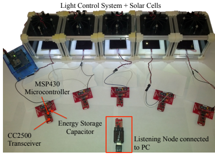
Fig. 4. Panda experimental setup: 5 EH nodes harvest energy through the solar cells with neighbor discovery rates monitored by a listening node.
