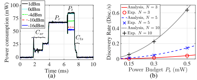
Fig. 5. (a) Power consumption for a node transitioning between the sleep, receive, and transmit states, and back to sleep. (b) Panda's discovery rate with varying power budgets, P_b , and number of nodes, N .
