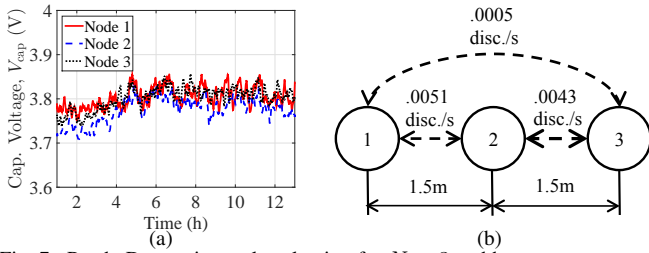
Fig. 7. Panda-D experimental evaluation for N = 3 and homogeneous power harvesting P_b = 0.15\text{mW} : (a) Capacitor voltage, V_{cap} , in a clique topology. (b) Per link experimental discovery rates for a line topology after 50 hours.
