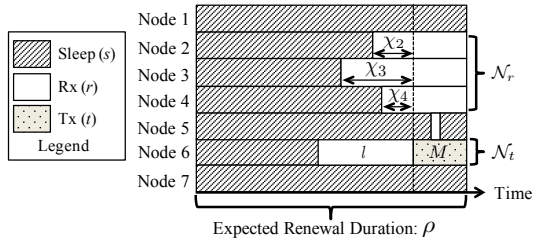
Fig. 2. Renewal process representing one renewal cycle for N = 7 nodes: all nodes begin in a memoryless sleep state and the renewal restarts after the first node to wake up completes its transmission.
