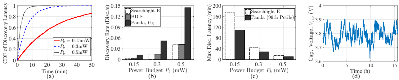
Fig. 6. Panda experimental evaluation for N = 5 : (a) CDF of per link discovery latency; comparison to SearchLight-E [10] and BD-E [12] of (b) the discovery rate and (c) the worst case latency; (d) capacitor voltage for a node with a 30mF capacitor and P_b = 0.5\text{mW} .
