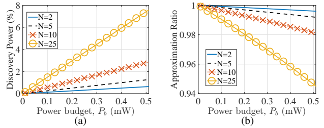
Fig. 3. The performance of the PCA for varying power budgets, P_b , and number of nodes, N : (a) discovery power as the percentage of the power budget ( \Phi(1)/P_b ), and (b) the approximation ratio ( U_A/\bar{U}^* ).
