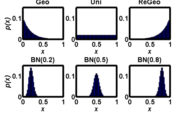
Figure 2: Common distributions: geometric, uniform, reversed geometric, binomial with p = 0.2, 0.5 and 0.8 .
